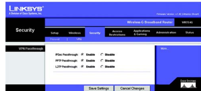
Figure 6-27 : Onglet Security - VPN Passthrough (Sécurité - Intercommunication VPN)
