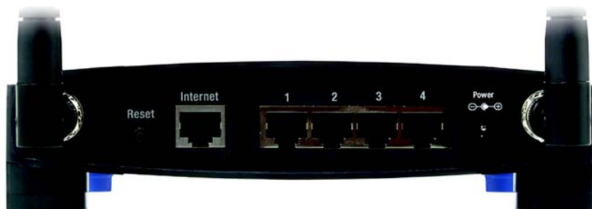
Figur 3-1: Routerns baksida
